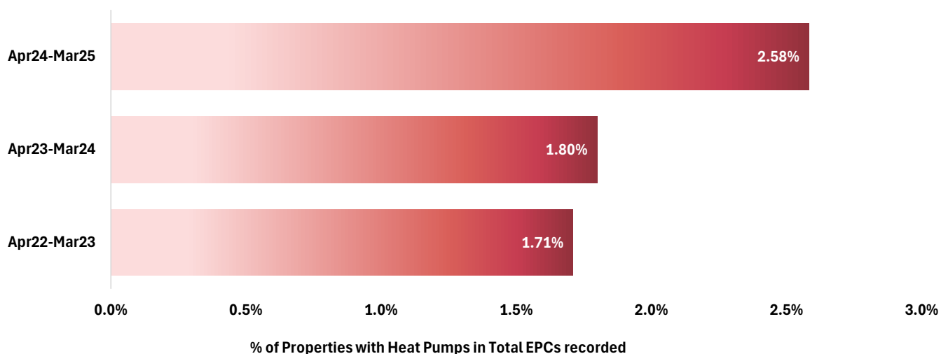
Trends in Heat Pumps recorded in EPCs issued (Apr22-Mar25)
