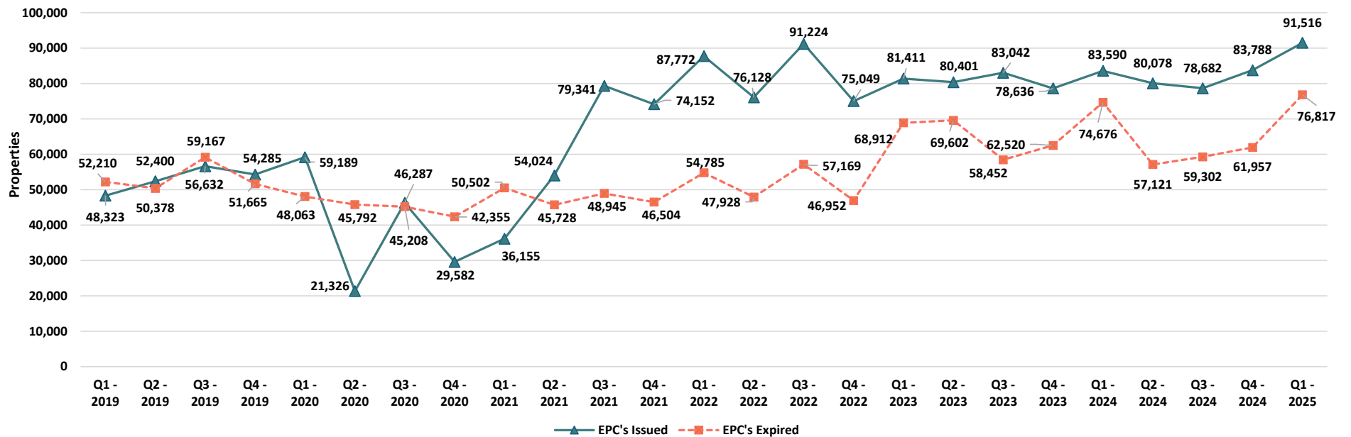
EPC's Issued vs. Expired (2019 - 2025)
