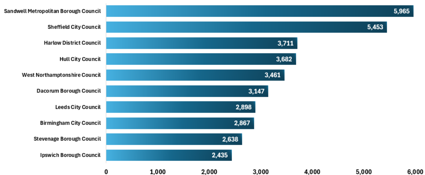
Local Authority issuing the most EPCs (April 2024 - March 2025)
